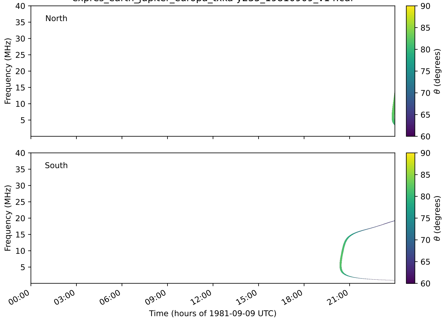
expres_earth_jupiter_europa_txka-y235_19810909_v14.cdf
