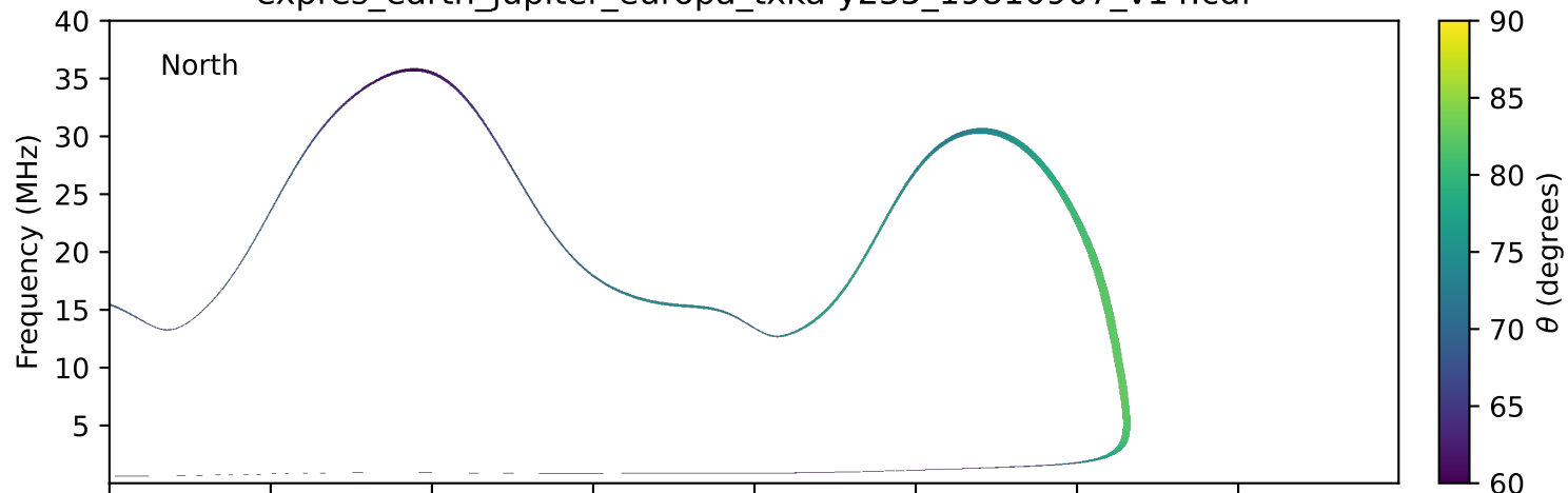
expres_earth_jupiter_europa_txka-y235_19810907_v14.cdf
