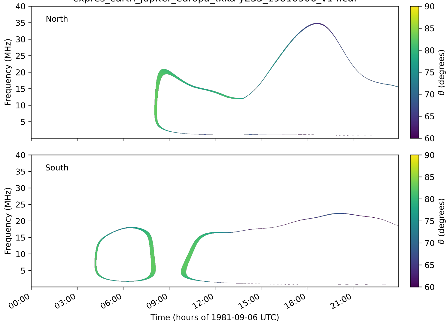
expres_earth_jupiter_europa_txka-y235_19810906_v14.cdf
