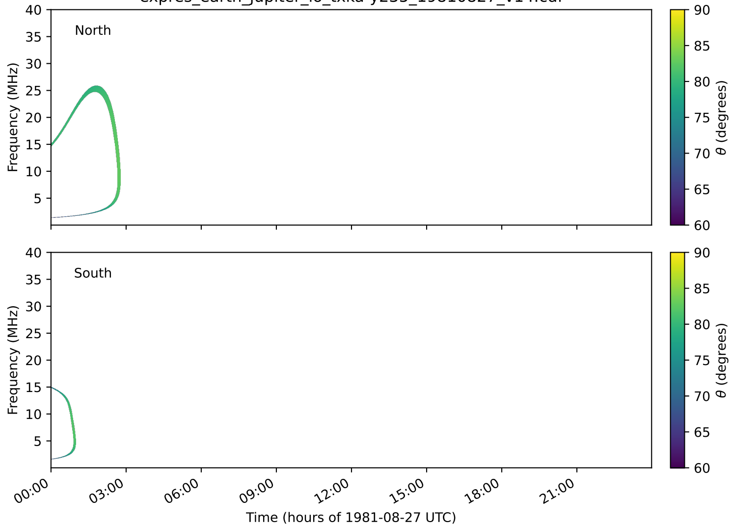
expres_earth_jupiter_io_txka-y235_19810827_v14.cdf
