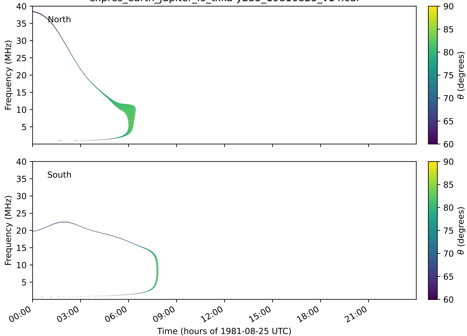
expres_earth_jupiter_io_txka-y235_19810825_v14.cdf
