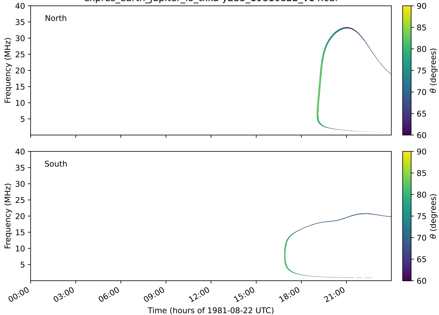
expres_earth_jupiter_io_txka-y235_19810822_v14.cdf
