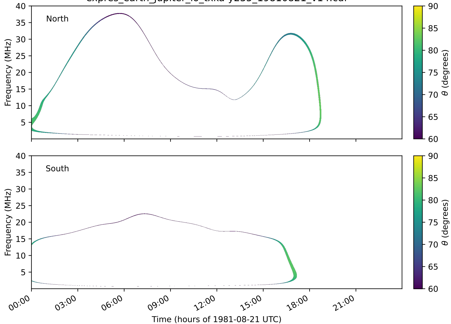
expres_earth_jupiter_io_txka-y235_19810821_v14.cdf
