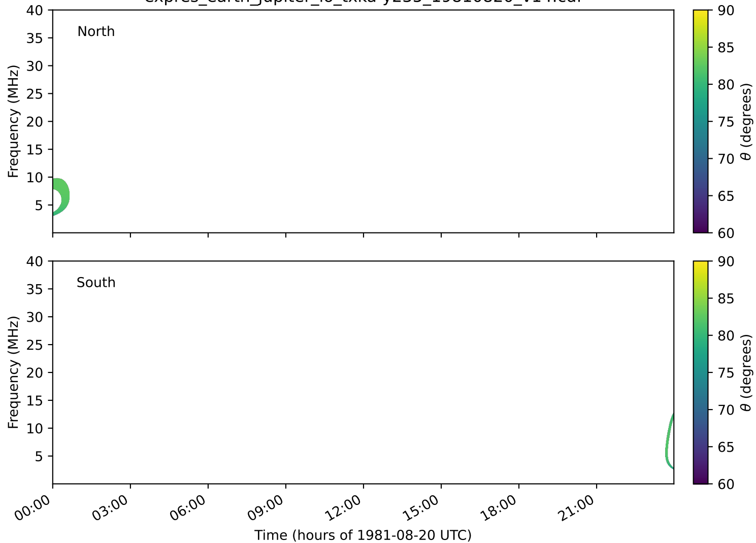
expres_earth_jupiter_io_txka-y235_19810820_v14.cdf
