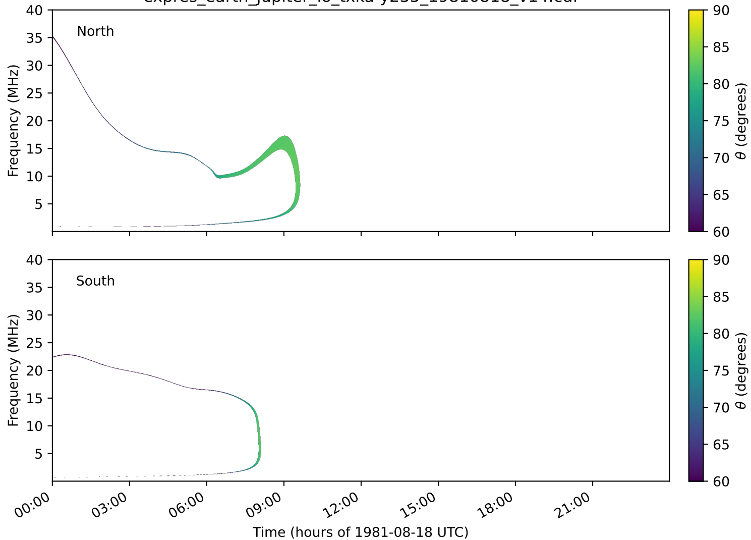
expres_earth_jupiter_io_txka-y235_19810818_v14.cdf
