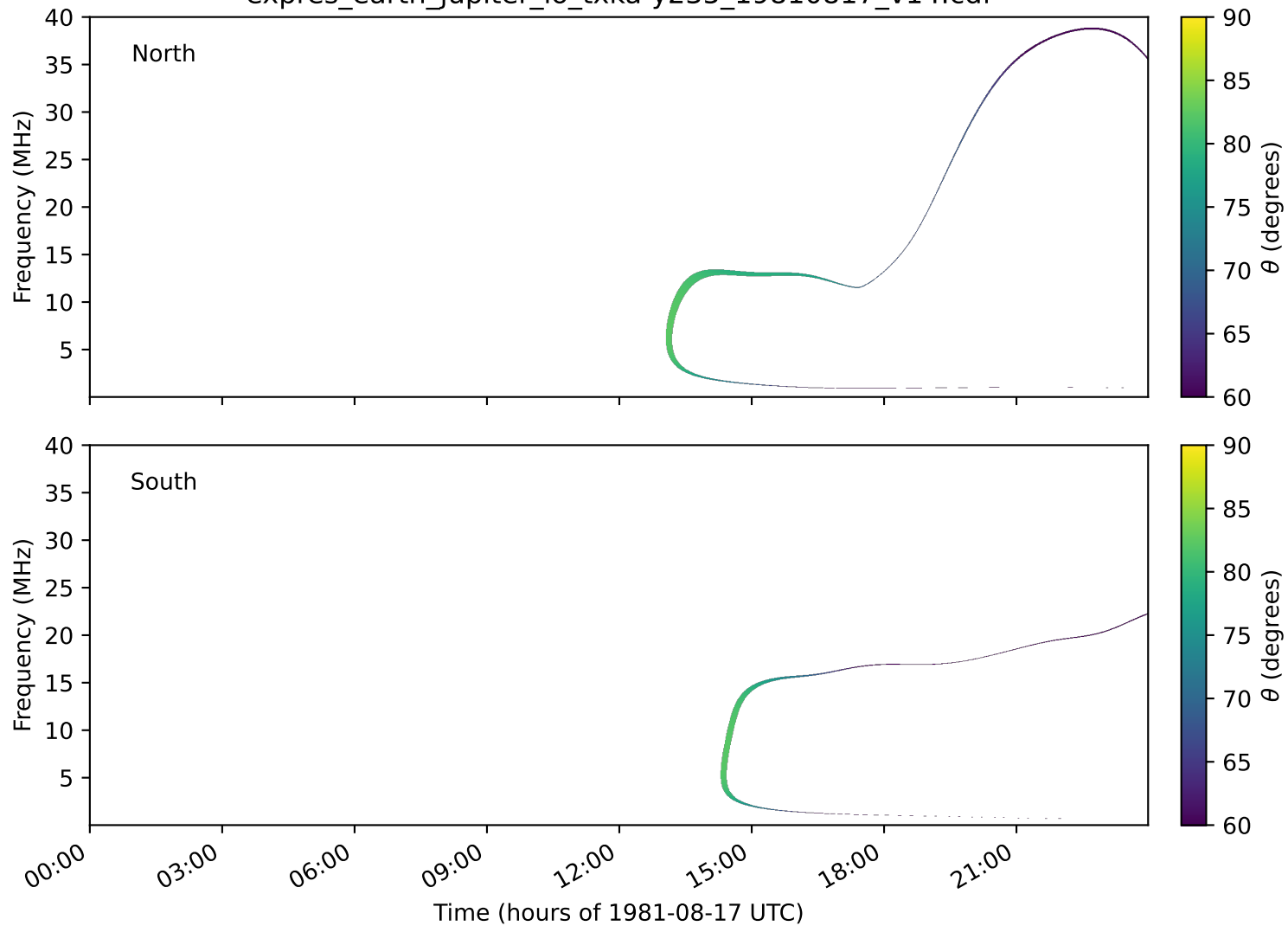
expres_earth_jupiter_io_txka-y235_19810817_v14.cdf
