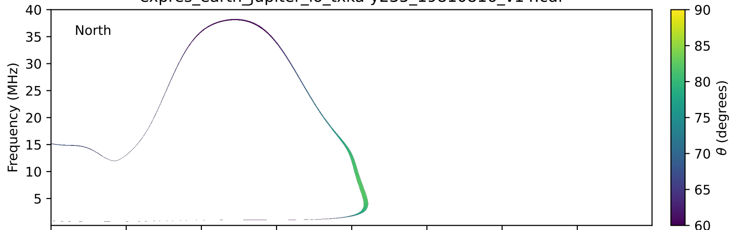
expres_earth_jupiter_io_txka-y235_19810816_v14.cdf
