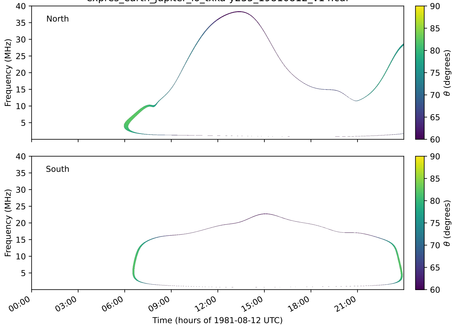
expres_earth_jupiter_io_txka-y235_19810812_v14.cdf
