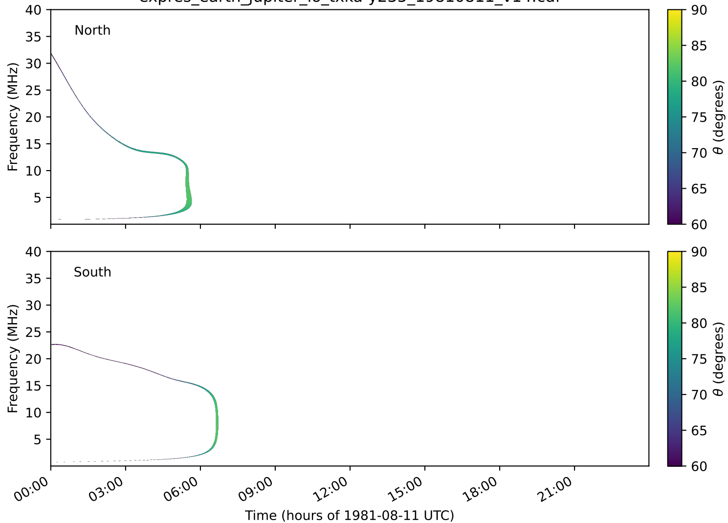
expres_earth_jupiter_io_txka-y235_19810811_v14.cdf
