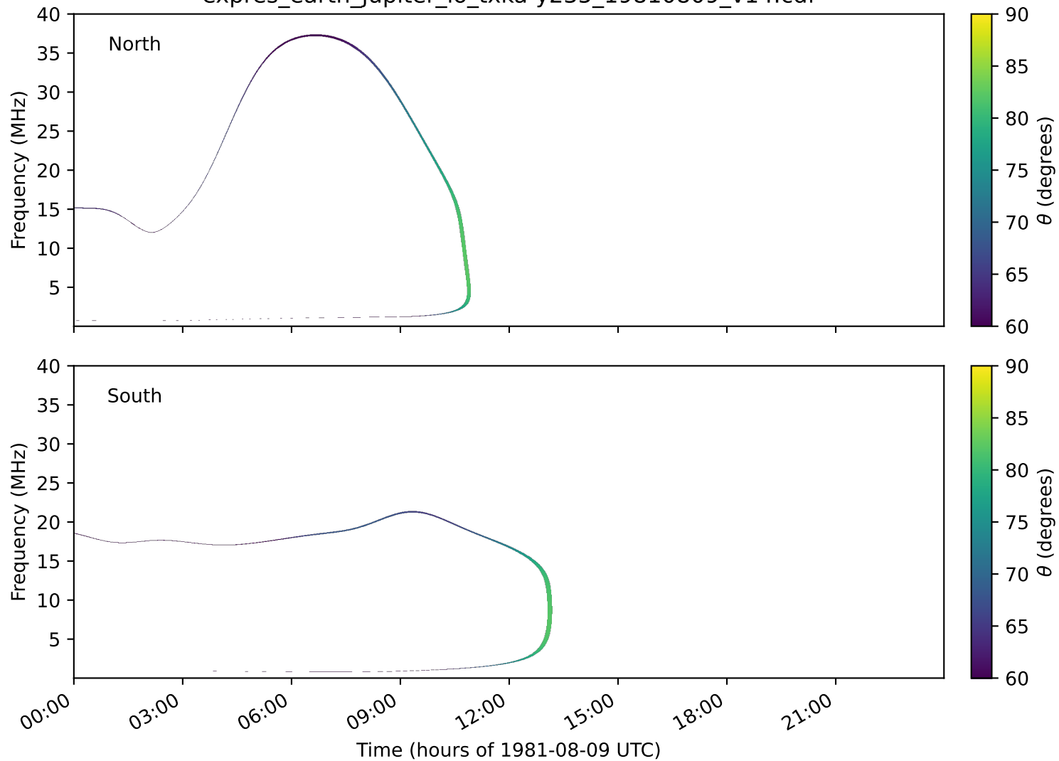
expres_earth_jupiter_io_txka-y235_19810809_v14.cdf
