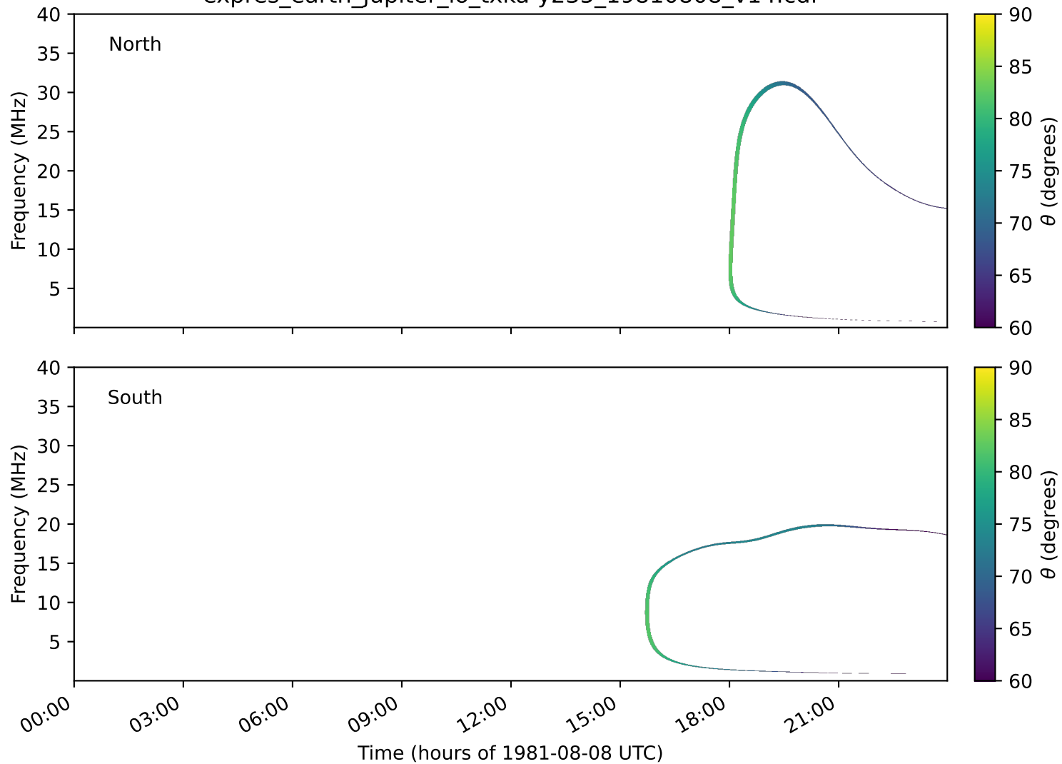
expres_earth_jupiter_io_txka-y235_19810808_v14.cdf
