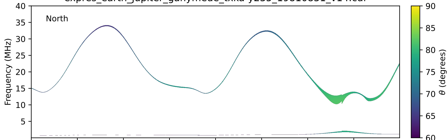
expres_earth_jupiter_ganymede_txka-y235_19810831_v14.cdf
