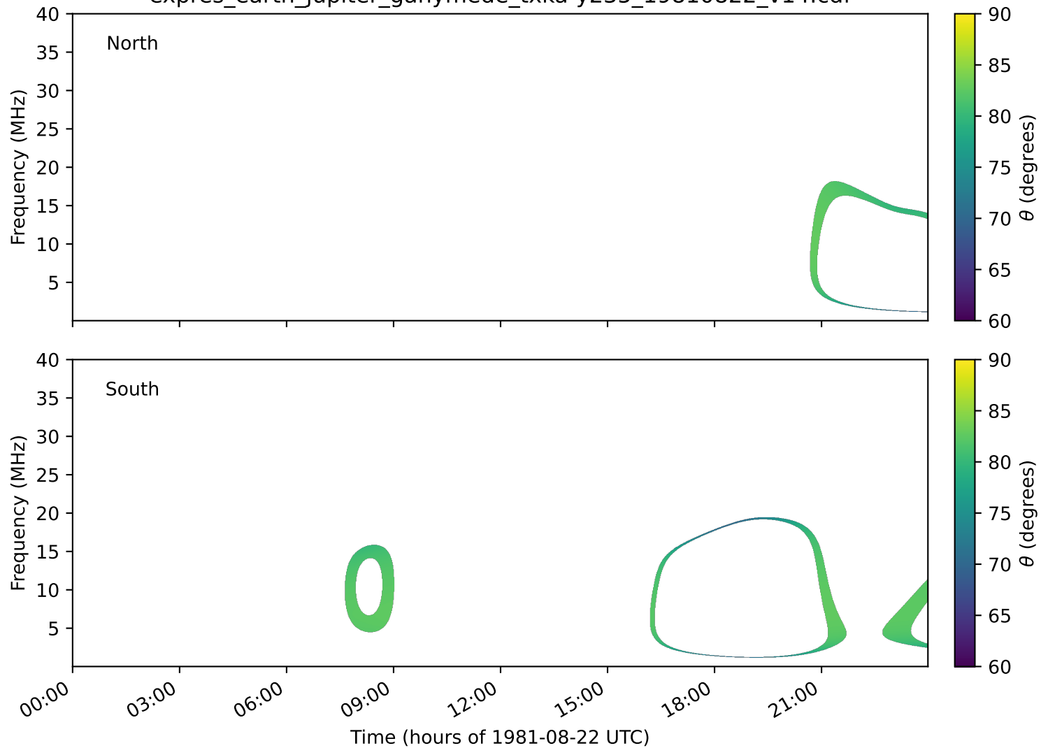
expres_earth_jupiter_ganymede_txka-y235_19810822_v14.cdf
