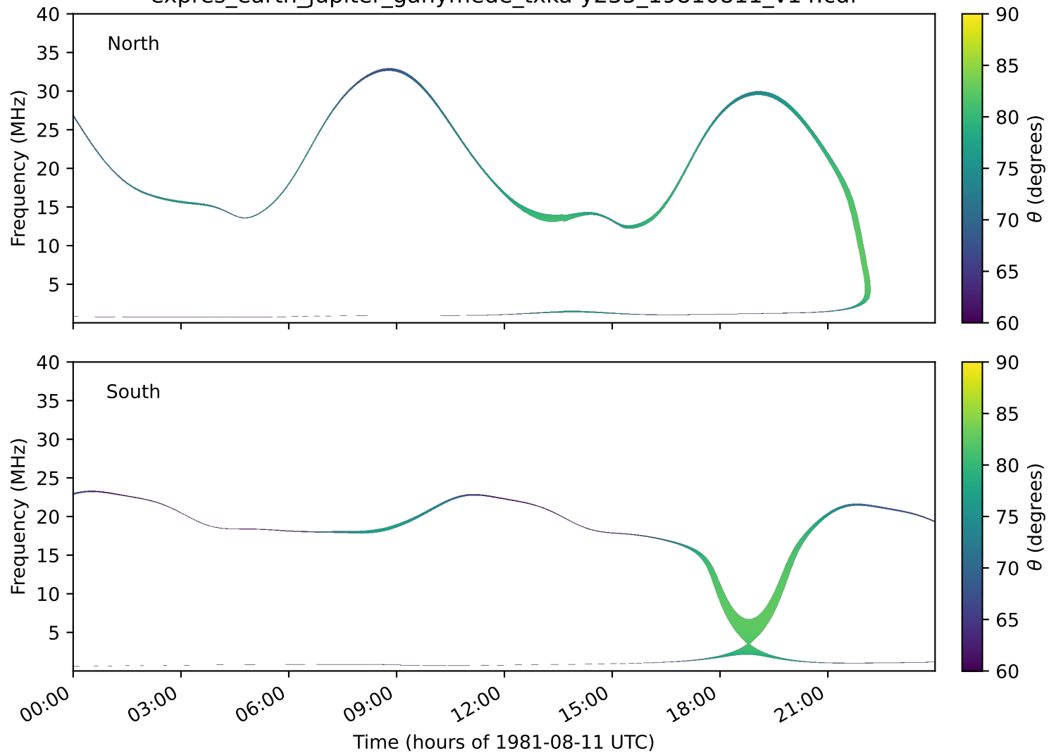
expres_earth_jupiter_ganymede_txka-y235_19810811_v14.cdf
