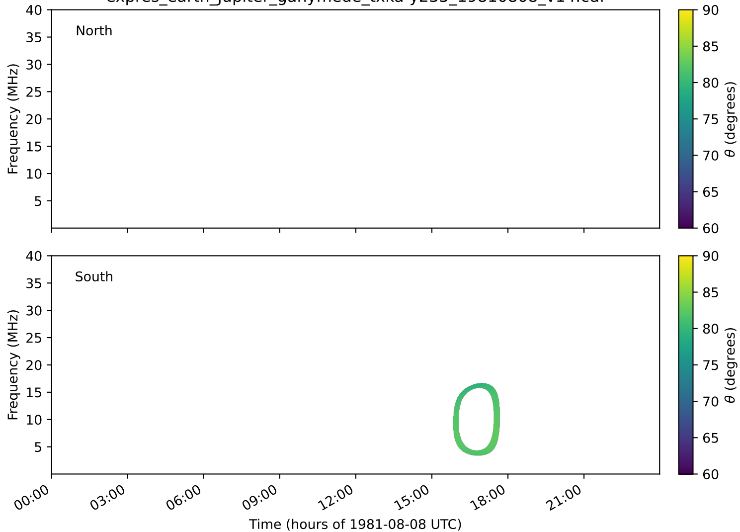
expres_earth_jupiter_ganymede_txka-y235_19810808_v14.cdf
