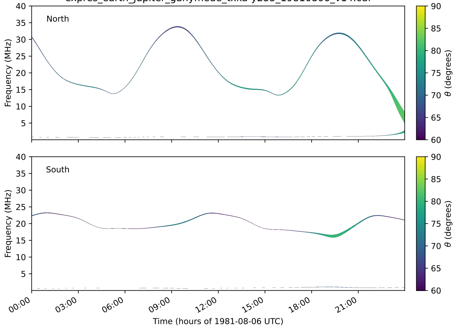
expres_earth_jupiter_ganymede_txka-y235_19810806_v14.cdf
