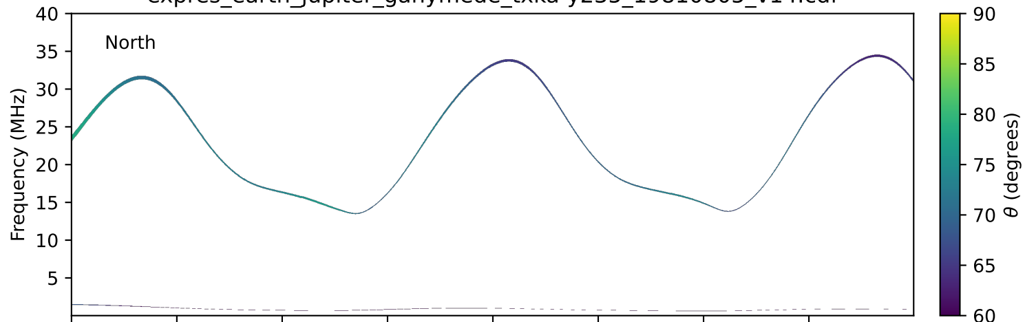
expres_earth_jupiter_ganymede_txka-y235_19810805_v14.cdf
