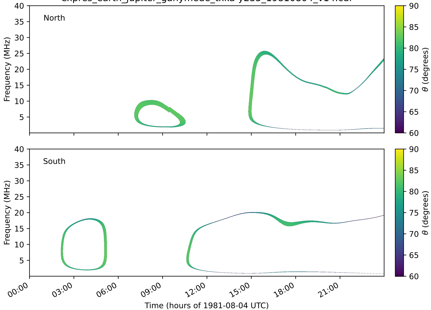
expres_earth_jupiter_ganymede_txka-y235_19810804_v14.cdf
