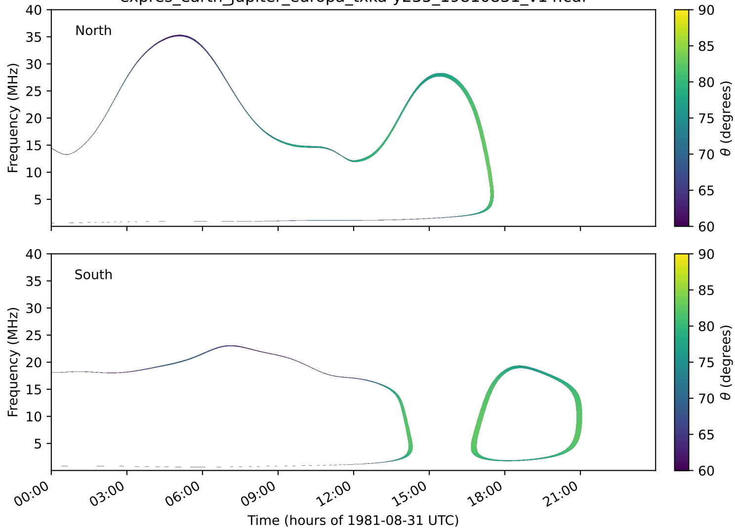
expres_earth_jupiter_europa_txka-y235_19810831_v14.cdf
