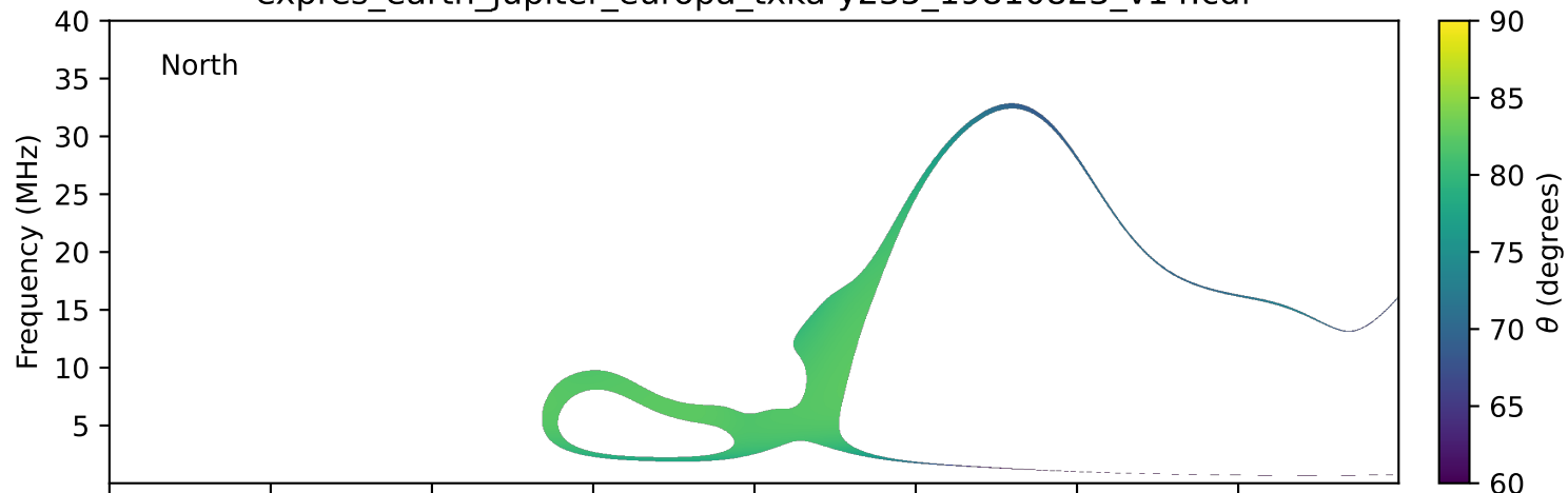
expres_earth_jupiter_europa_txka-y235_19810823_v14.cdf
