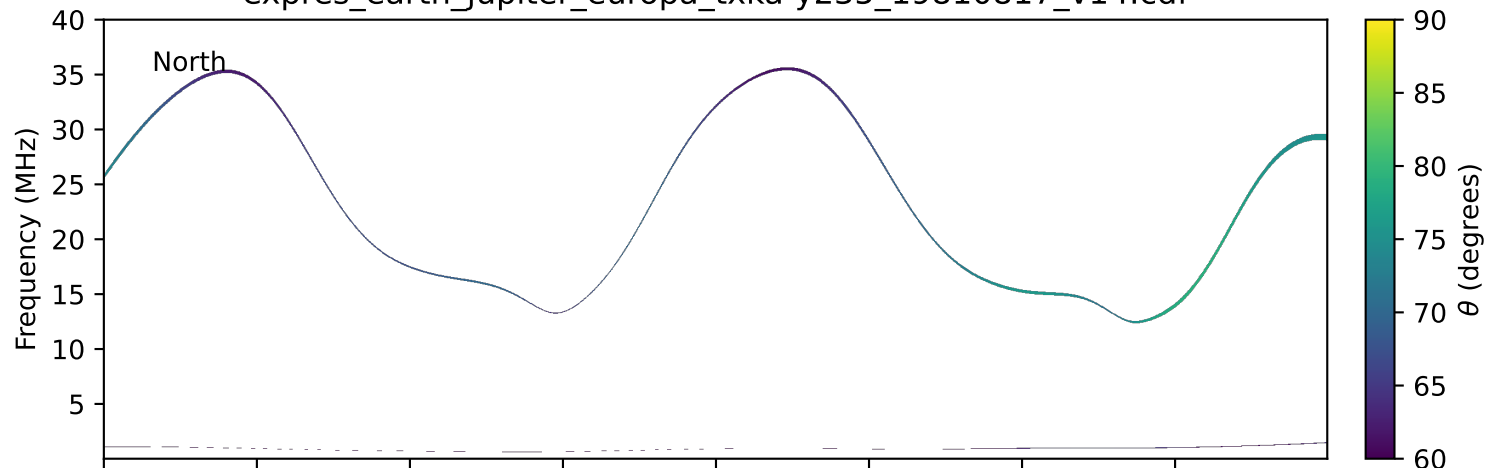
expres_earth_jupiter_europa_txka-y235_19810817_v14.cdf
