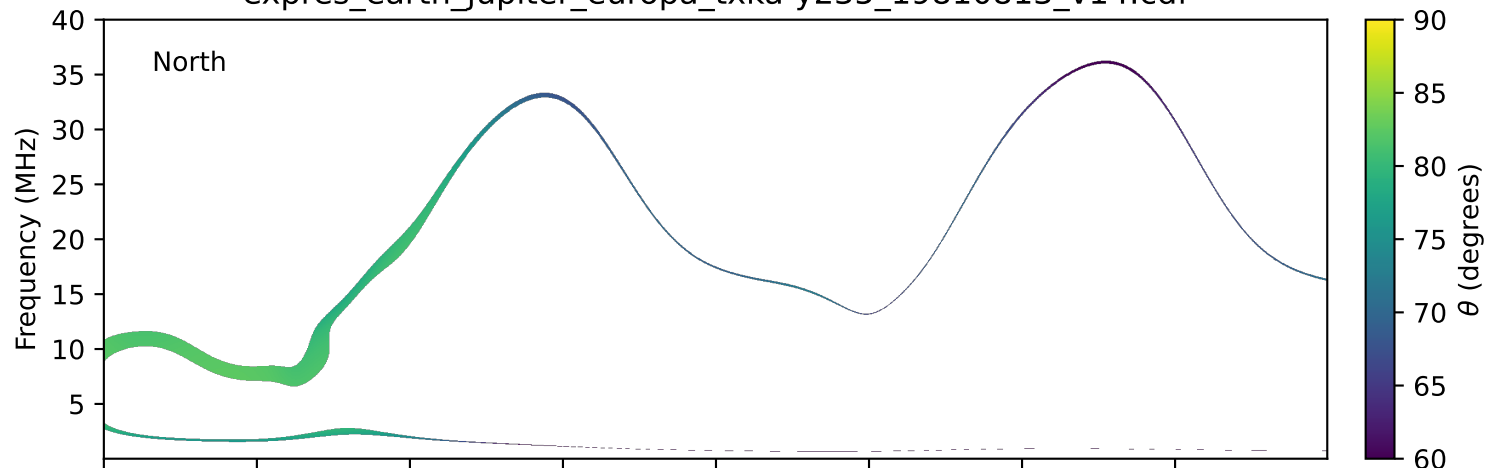
expres_earth_jupiter_europa_txka-y235_19810813_v14.cdf
