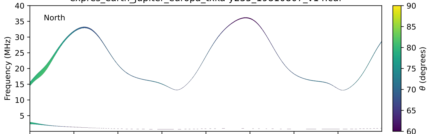
expres_earth_jupiter_europa_txka-y235_19810807_v14.cdf
