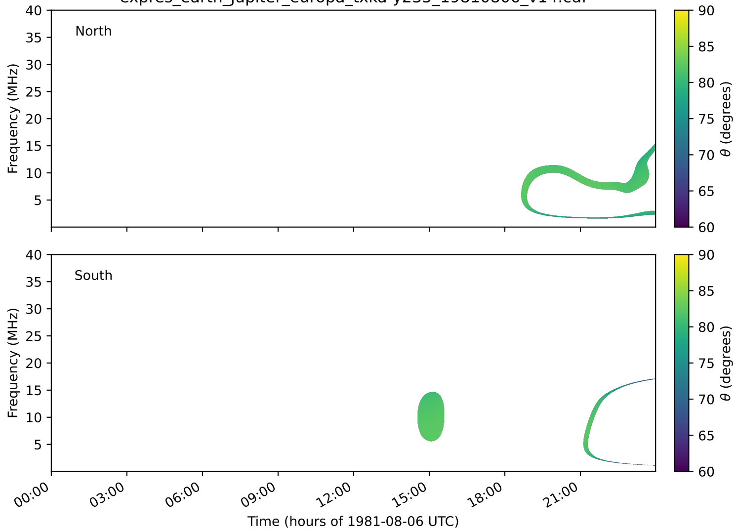
expres_earth_jupiter_europa_txka-y235_19810806_v14.cdf
