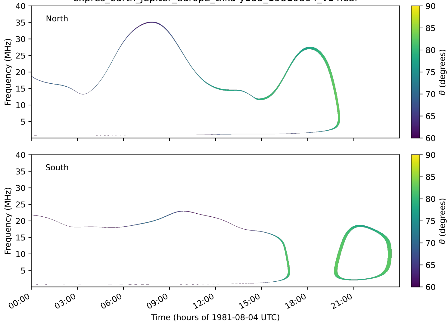
expres_earth_jupiter_europa_txka-y235_19810804_v14.cdf
