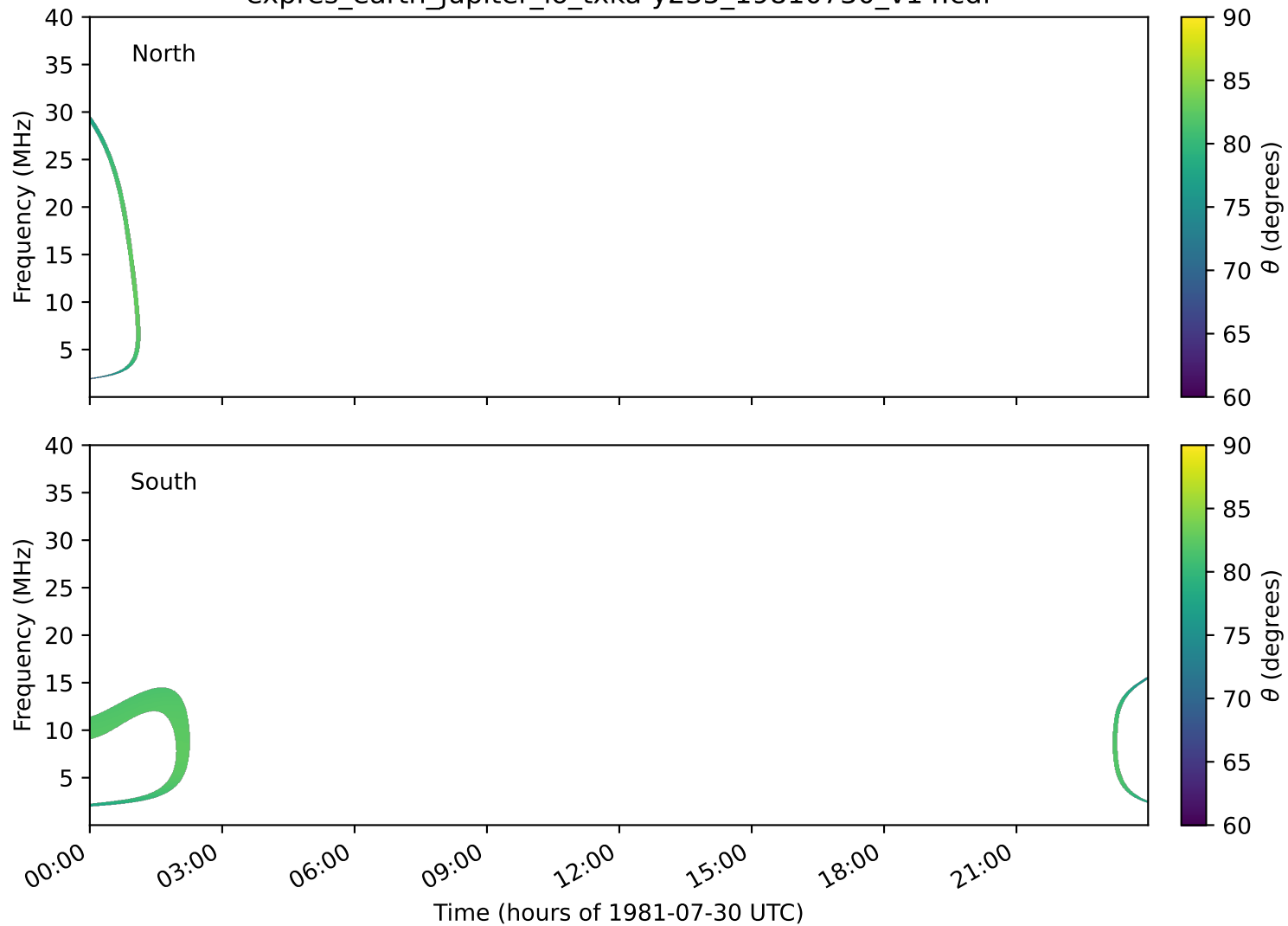
expres_earth_jupiter_io_txka-y235_19810730_v14.cdf
