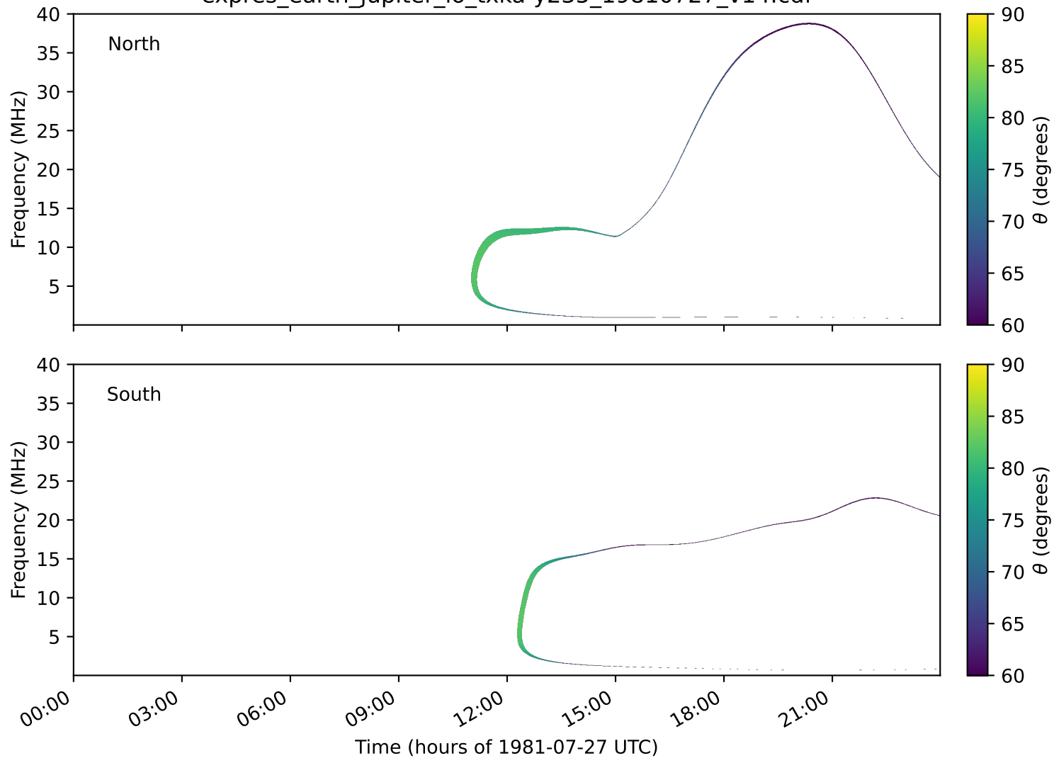
expres_earth_jupiter_io_txka-y235_19810727_v14.cdf
