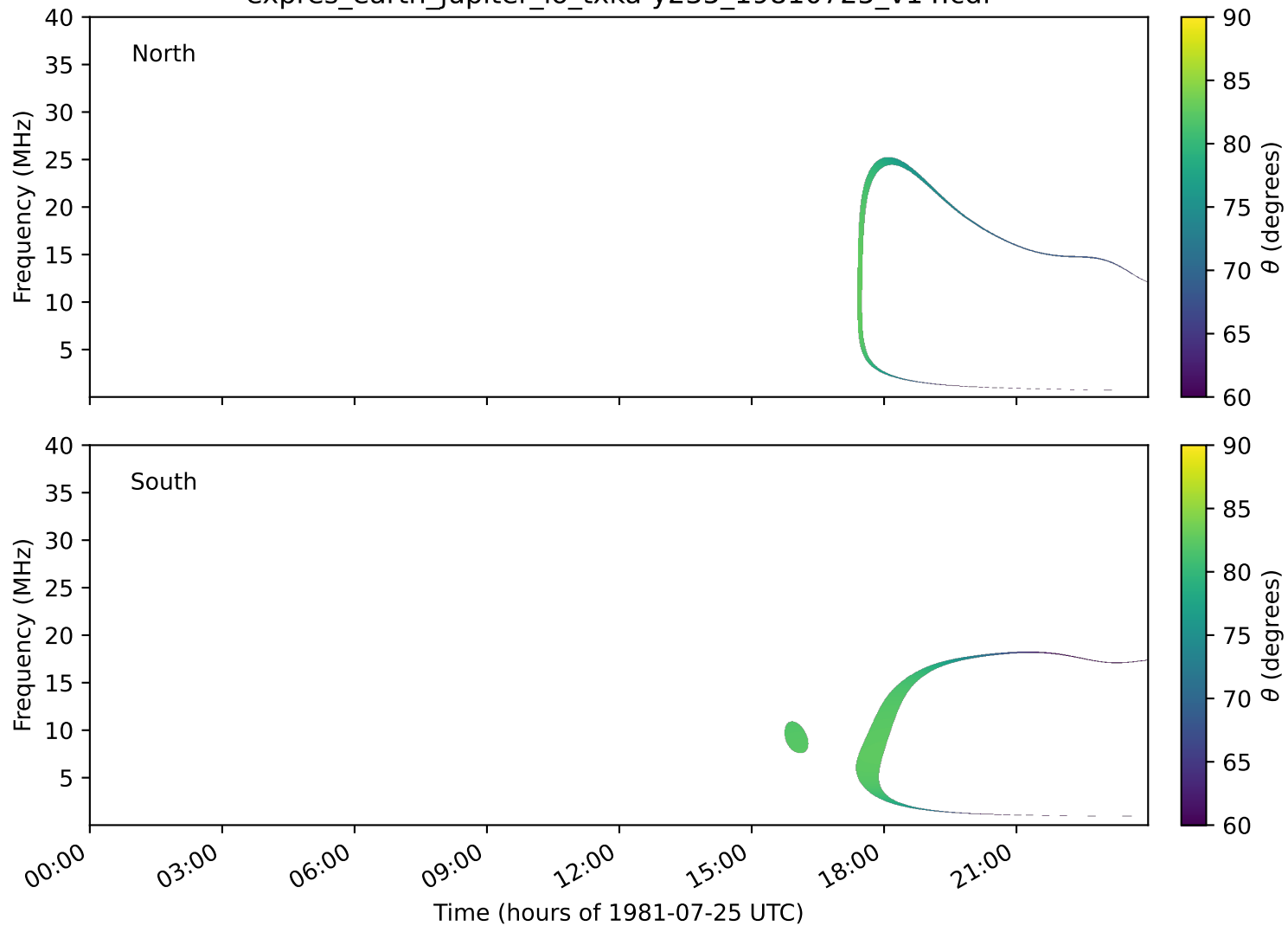
expres_earth_jupiter_io_txka-y235_19810725_v14.cdf
