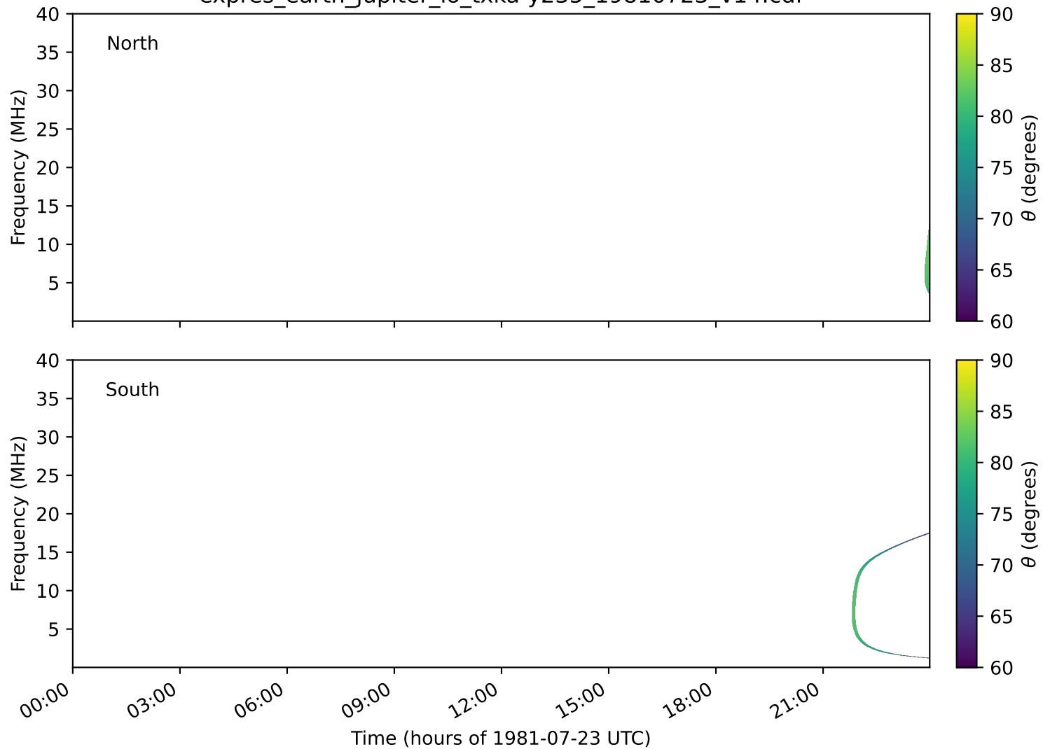
expres_earth_jupiter_io_txka-y235_19810723_v14.cdf
