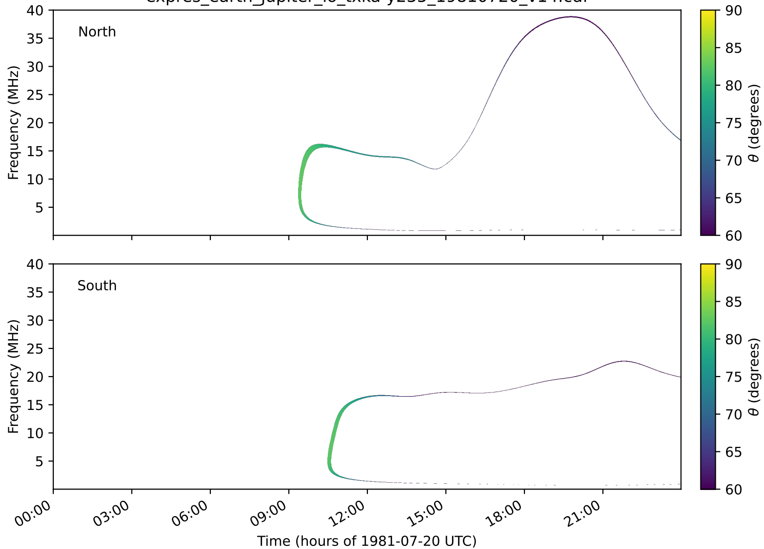
expres_earth_jupiter_io_txka-y235_19810720_v14.cdf
