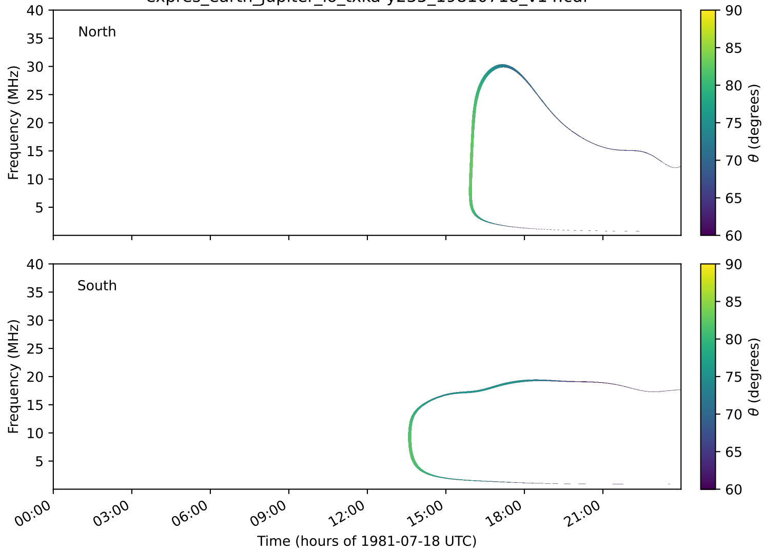
expres_earth_jupiter_io_txka-y235_19810718_v14.cdf
