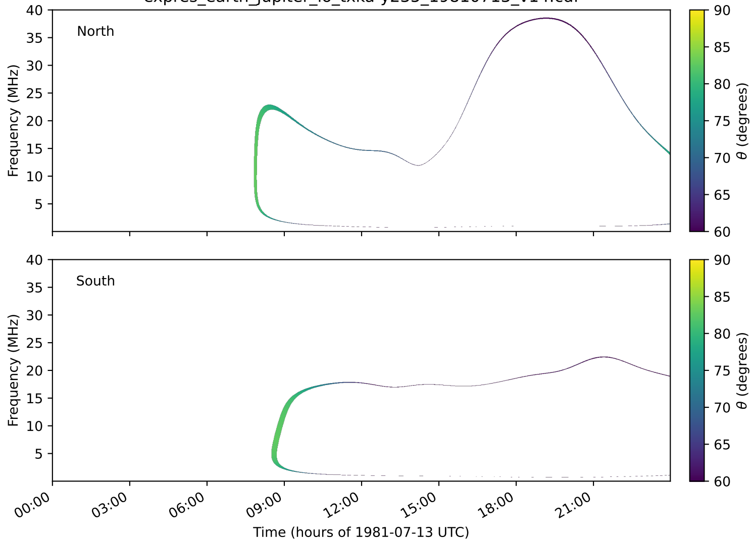
expres_earth_jupiter_io_txka-y235_19810713_v14.cdf
