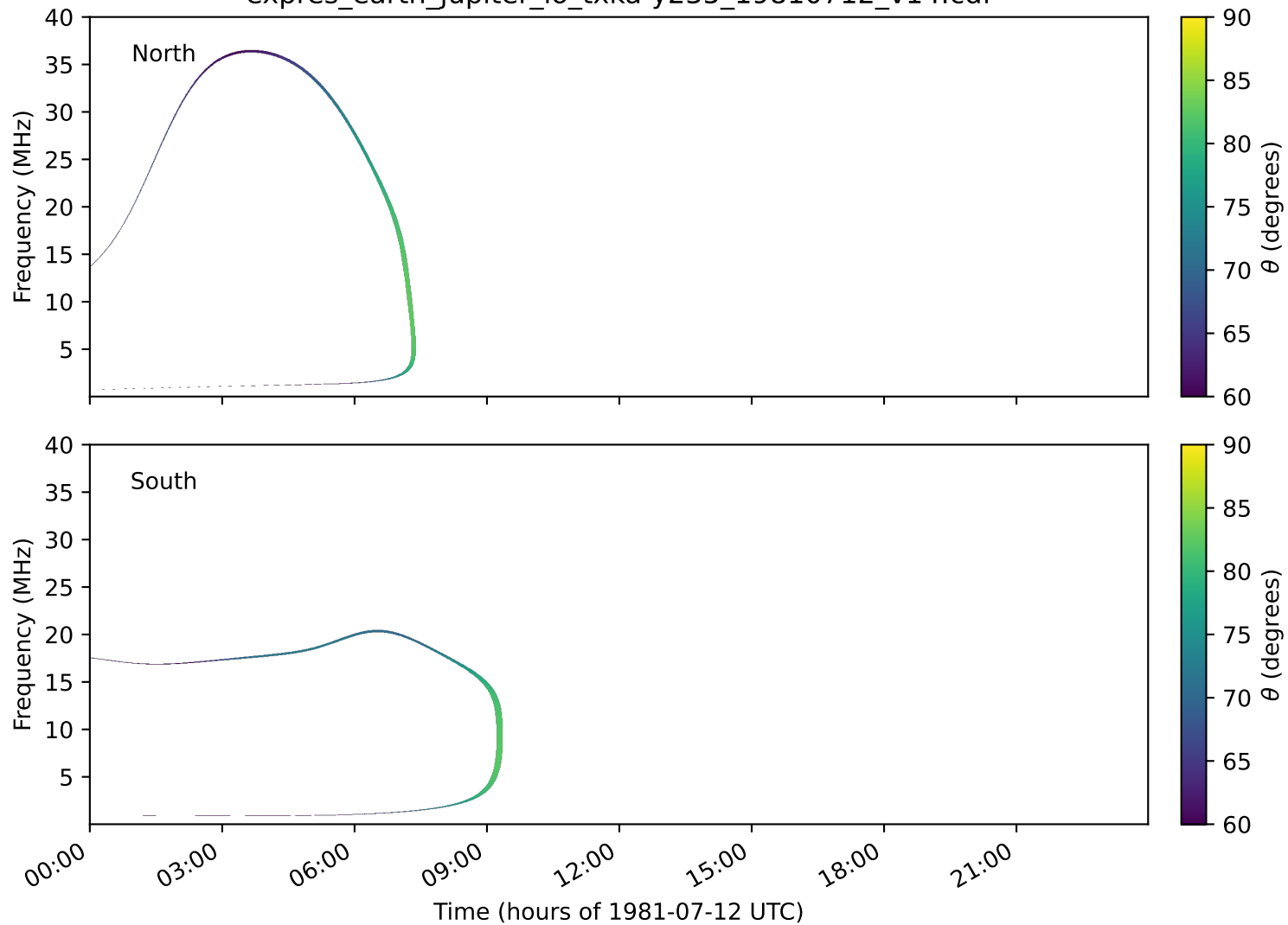
expres_earth_jupiter_io_txka-y235_19810712_v14.cdf
