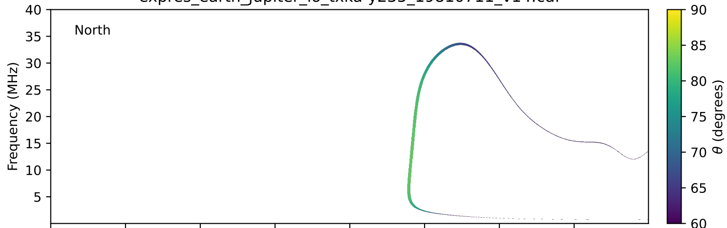
expres_earth_jupiter_io_txka-y235_19810711_v14.cdf
