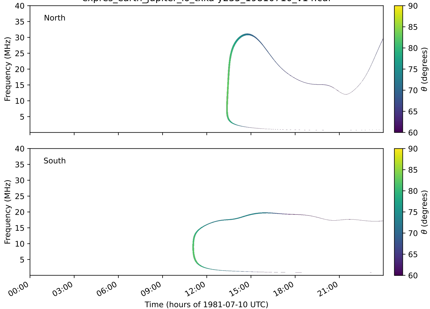
expres_earth_jupiter_io_txka-y235_19810710_v14.cdf
