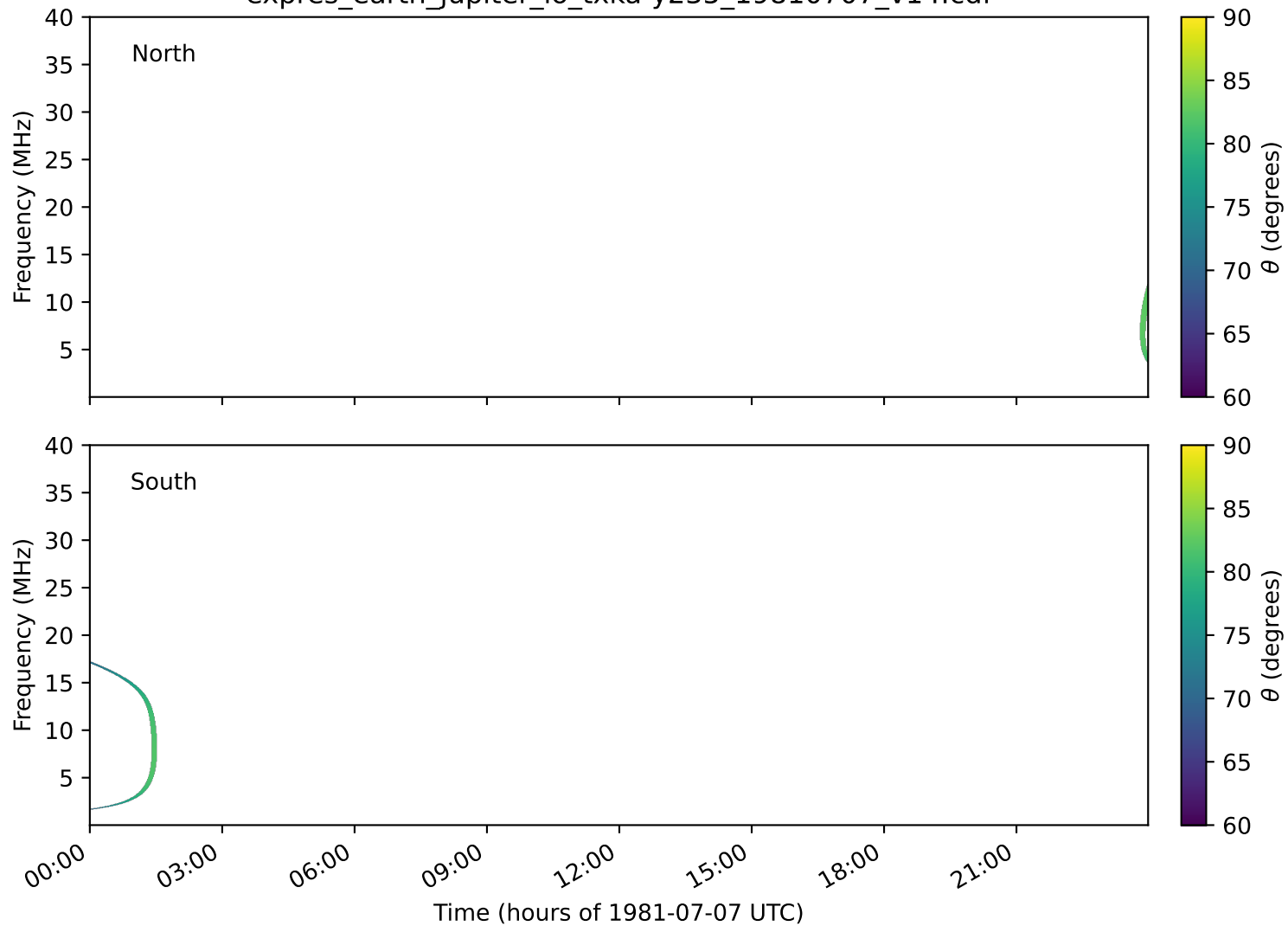
expres_earth_jupiter_io_txka-y235_19810707_v14.cdf
