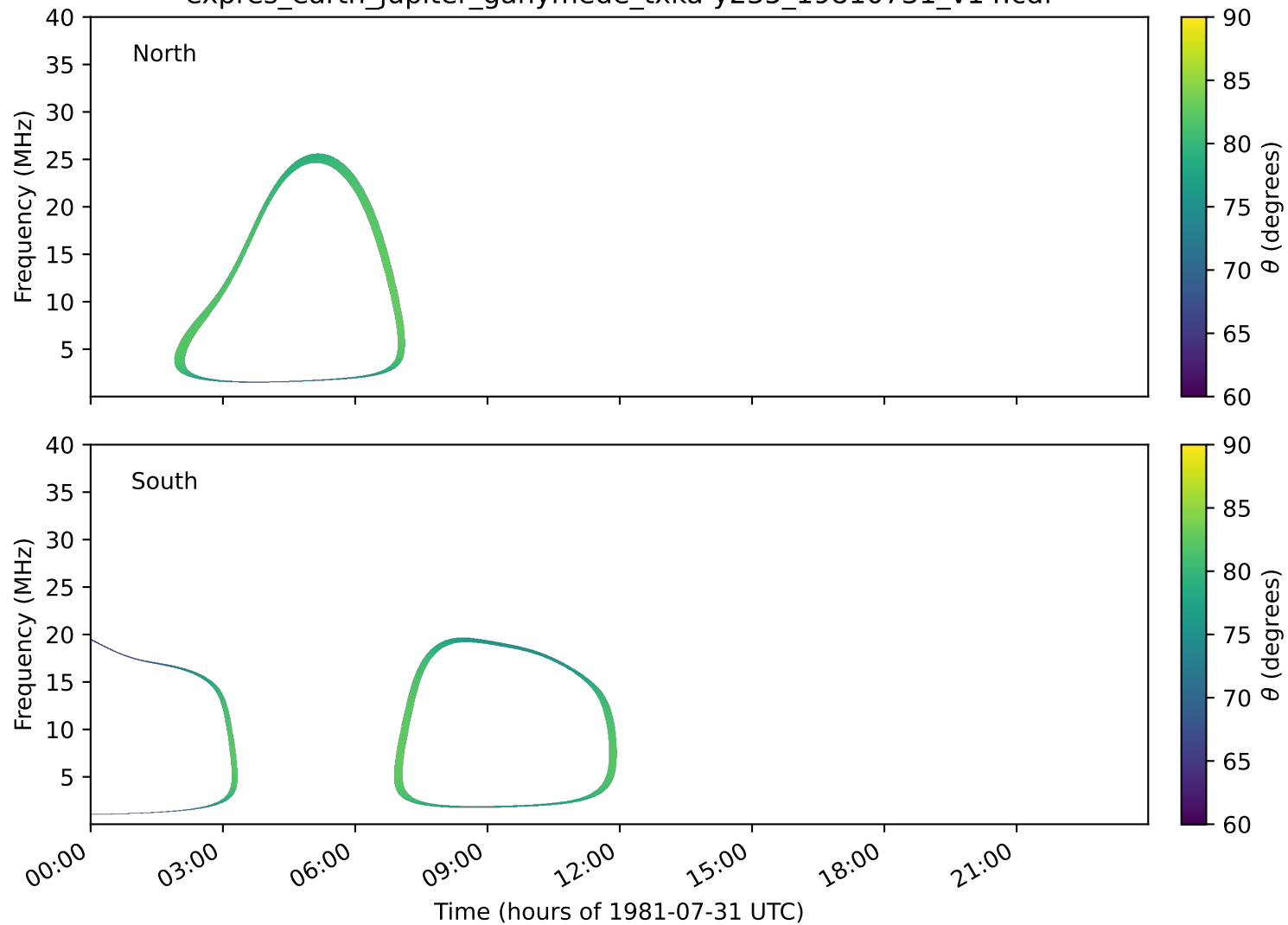
expres_earth_jupiter_ganymede_txka-y235_19810731_v14.cdf
