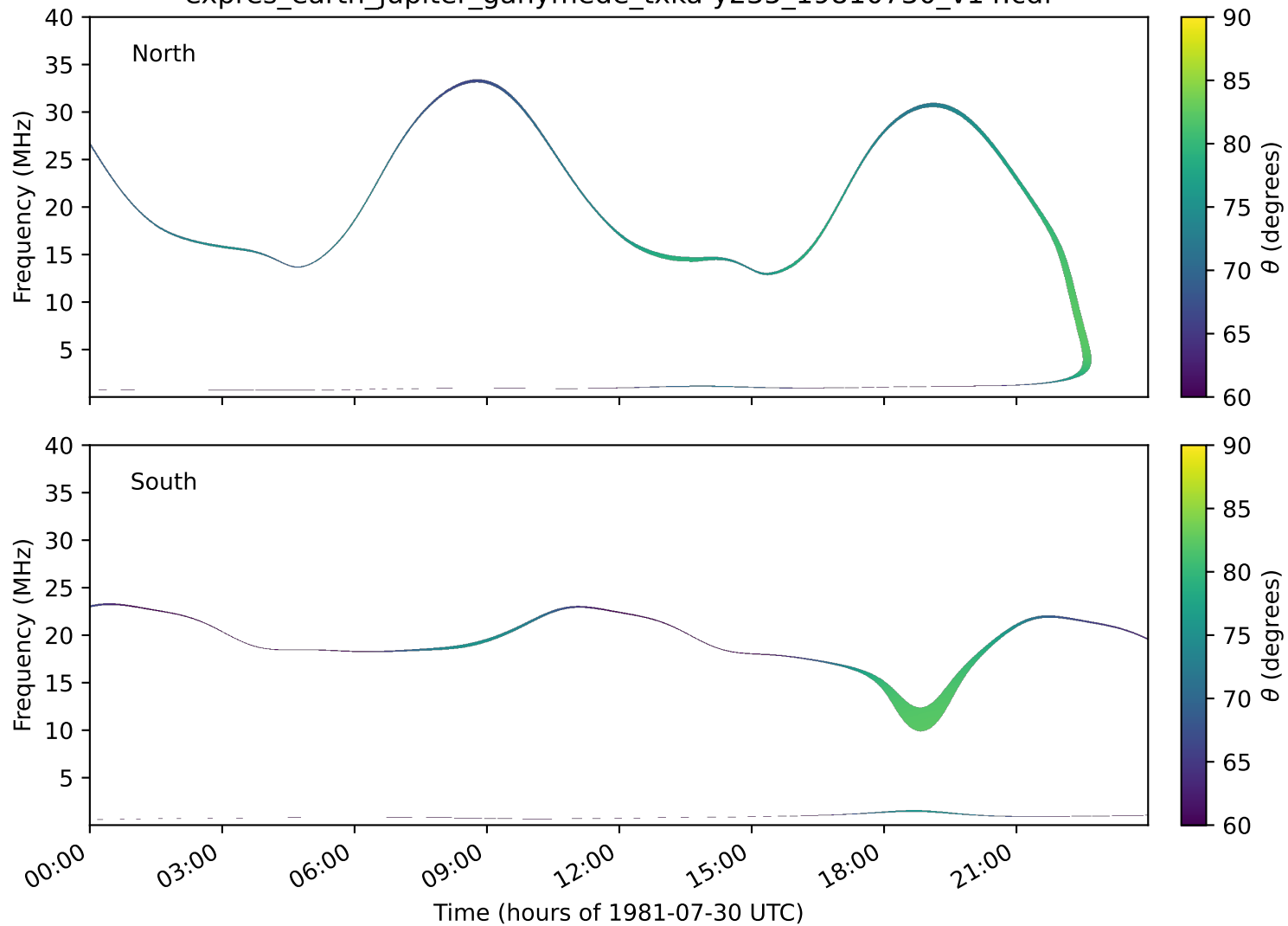
expres_earth_jupiter_ganymede_txka-y235_19810730_v14.cdf
