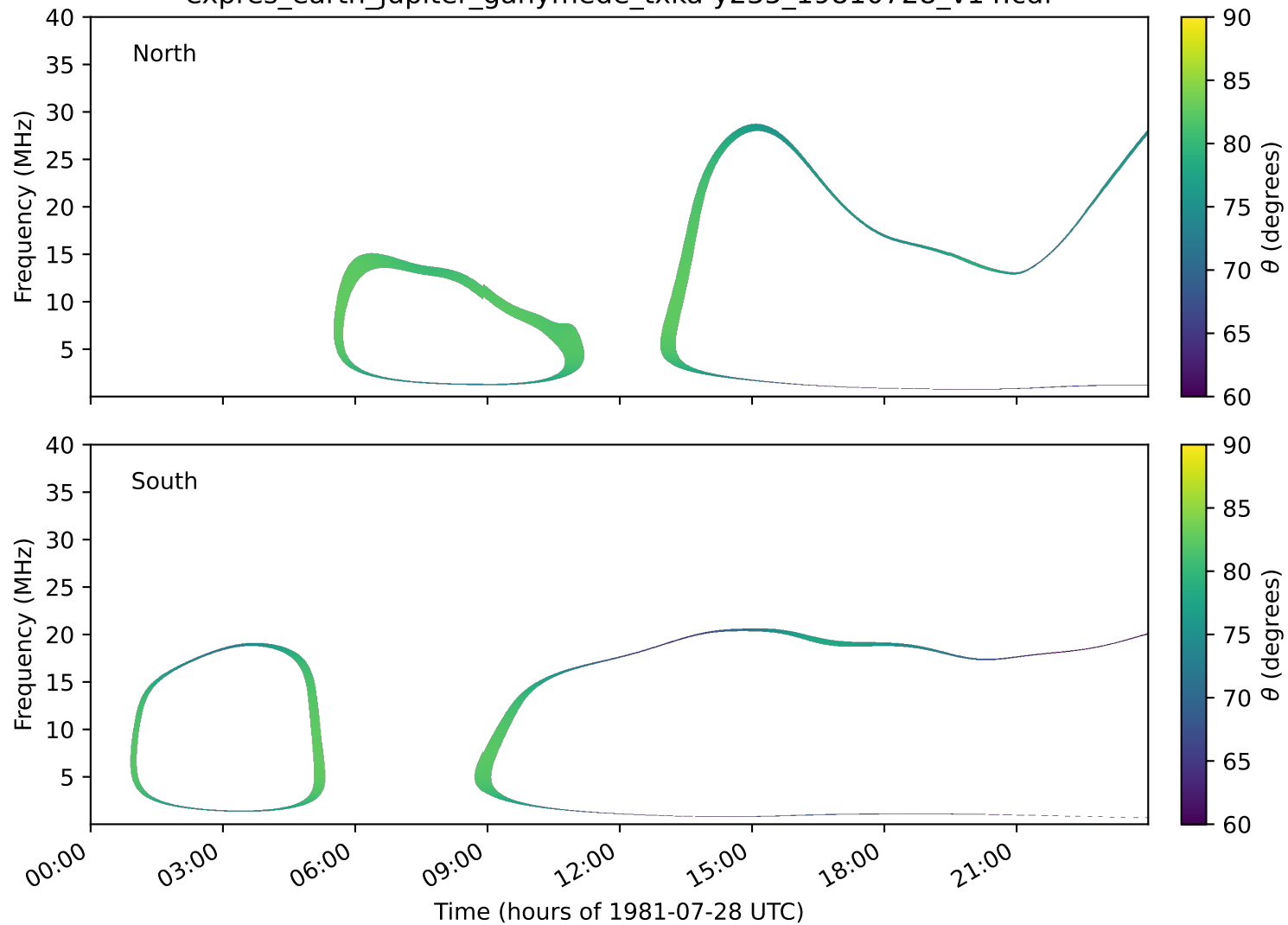
expres_earth_jupiter_ganymede_txka-y235_19810728_v14.cdf
