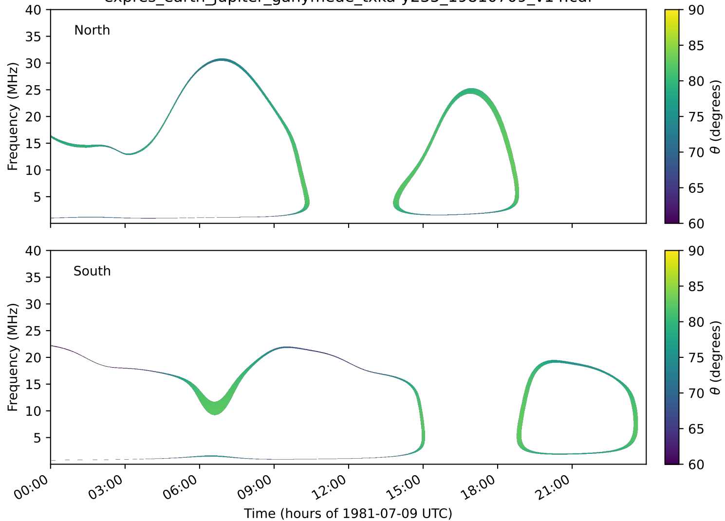
expres_earth_jupiter_ganymede_txka-y235_19810709_v14.cdf
