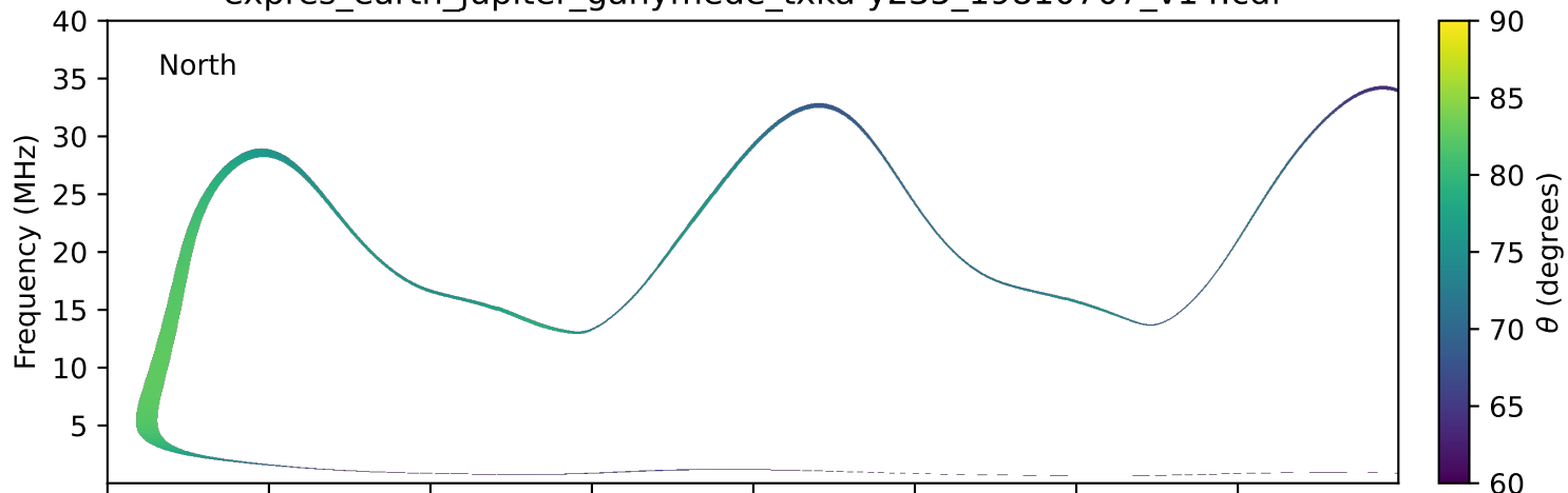
expres_earth_jupiter_ganymede_txka-y235_19810707_v14.cdf
