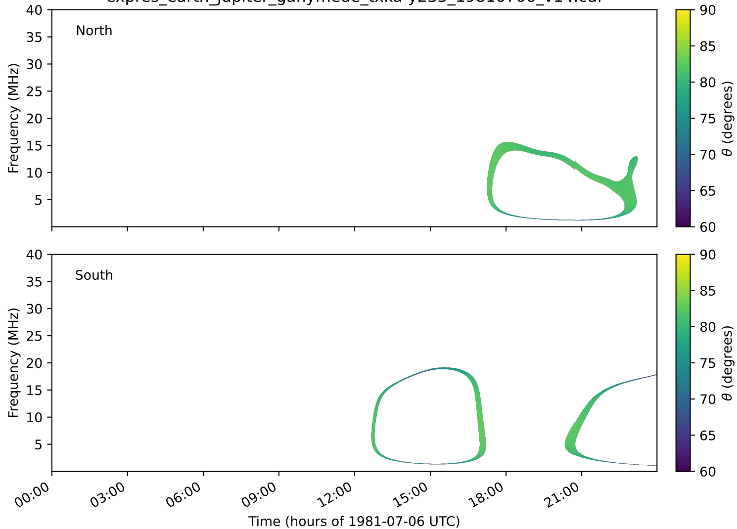
expres_earth_jupiter_ganymede_txka-y235_19810706_v14.cdf
