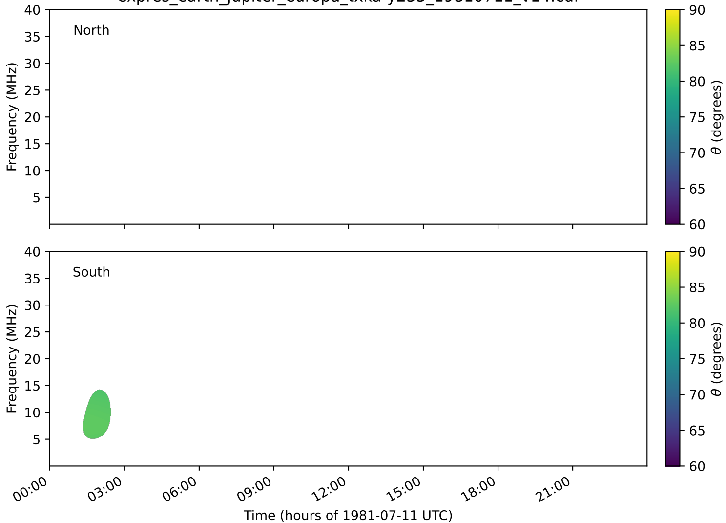
expres_earth_jupiter_europa_txka-y235_19810711_v14.cdf
