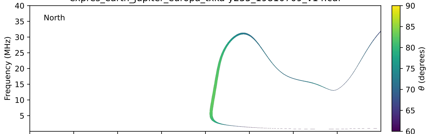
expres_earth_jupiter_europa_txka-y235_19810709_v14.cdf
