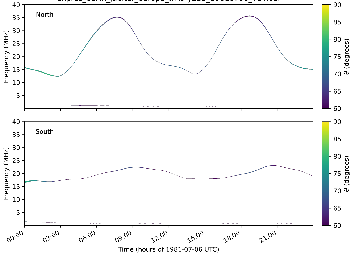
expres_earth_jupiter_europa_txka-y235_19810706_v14.cdf
