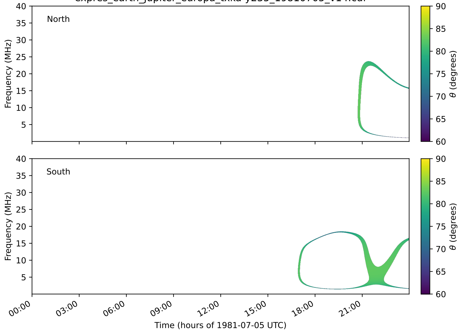
expres_earth_jupiter_europa_txka-y235_19810705_v14.cdf
